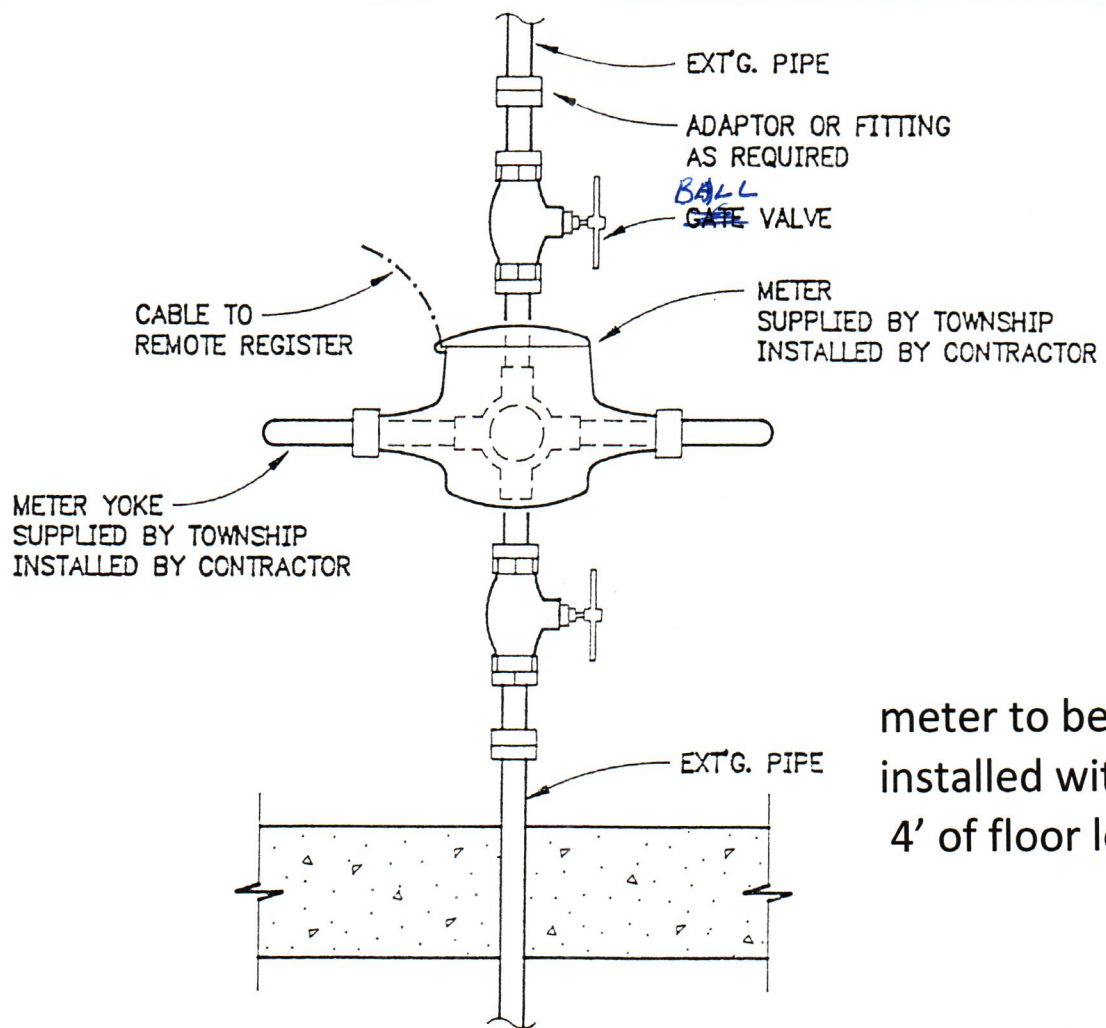
TYPICAL METER INSTALLATION METER YOKE SETTING
