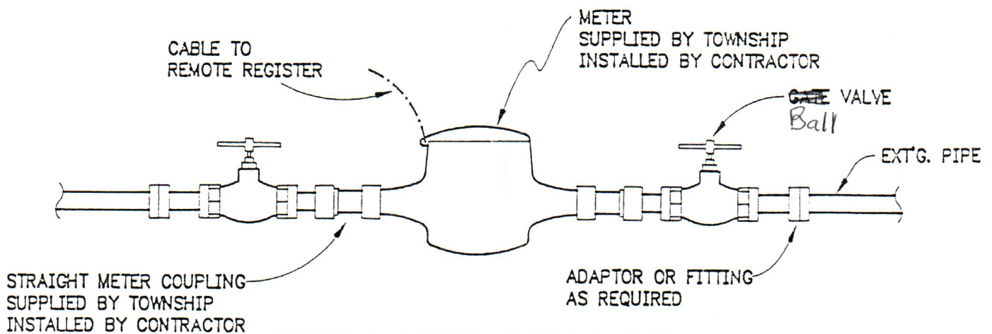
TYPICAL METER INSTALLATION STRAIGHT SETTING
