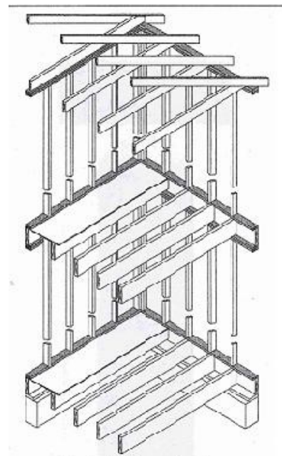
Typical Platform Framing Fireblocking shown in grey
