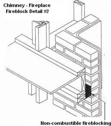
Non-combustible fireblocking
