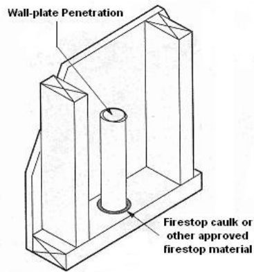
Typical Wall-plate Firestopping Detail
