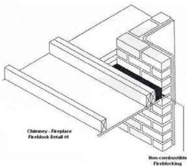
Non-combustible Fireblocking
