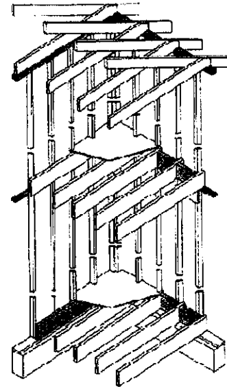
Typical Balloon Framing Fireblocking shown in grey areas
