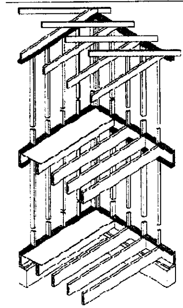
Typical Platform Framing Fireblocking shown in grey
