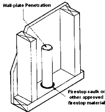
Typical Wall-plate Firestopping Detail
